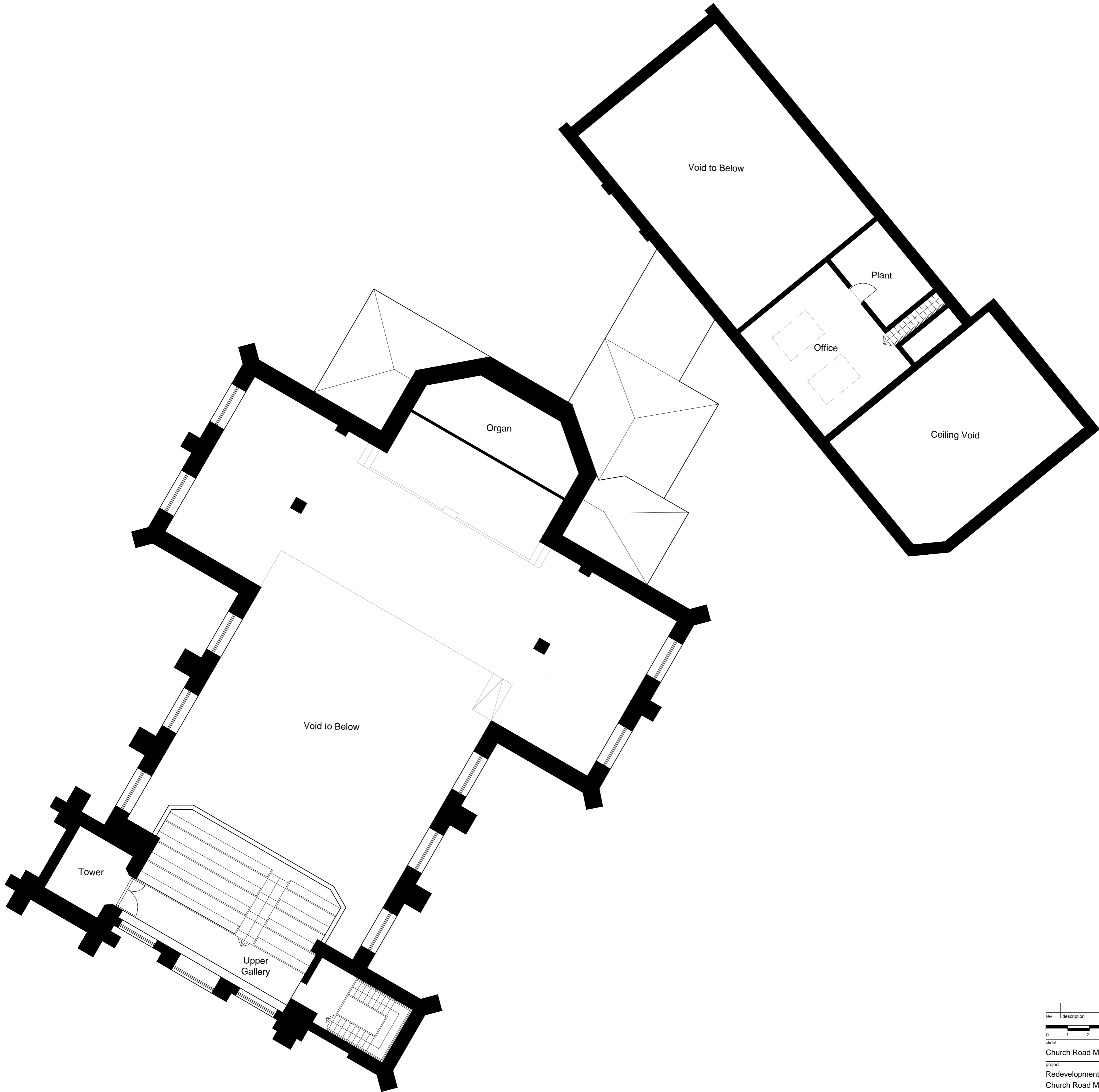
Upper Floor (1:100)
